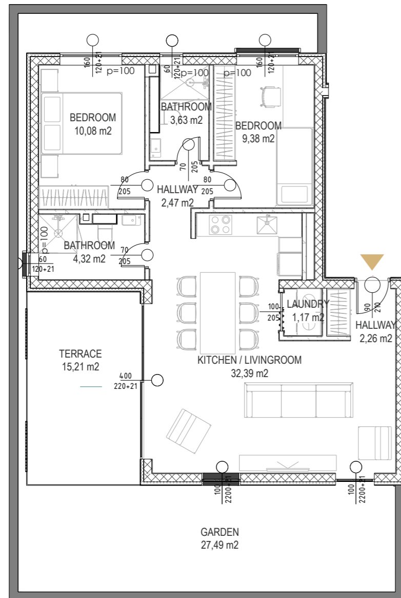
PLAN
