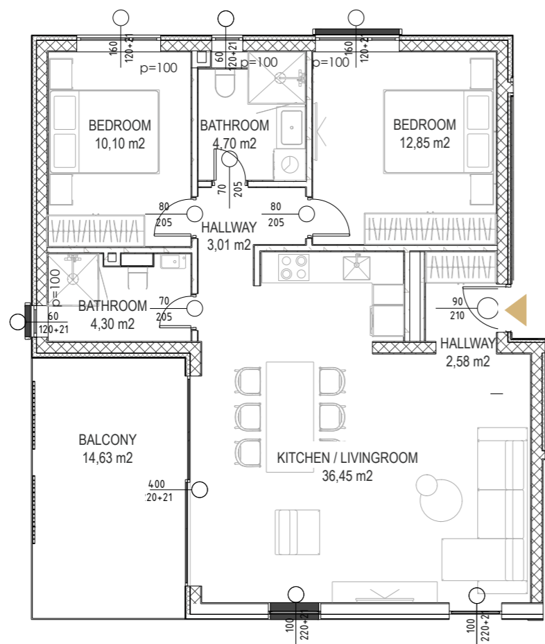
PLAN
