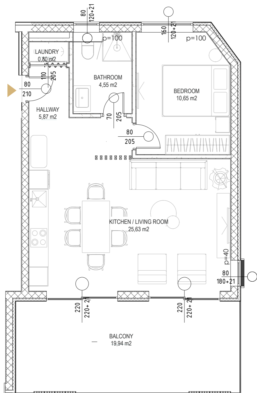
PLAN
