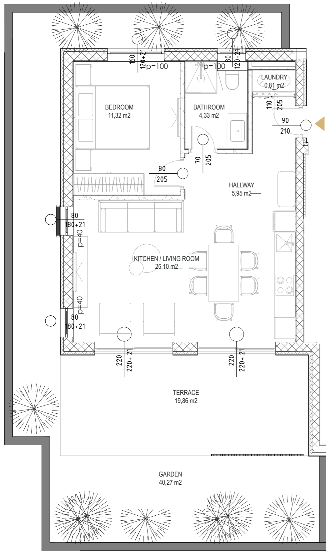
PLAN
