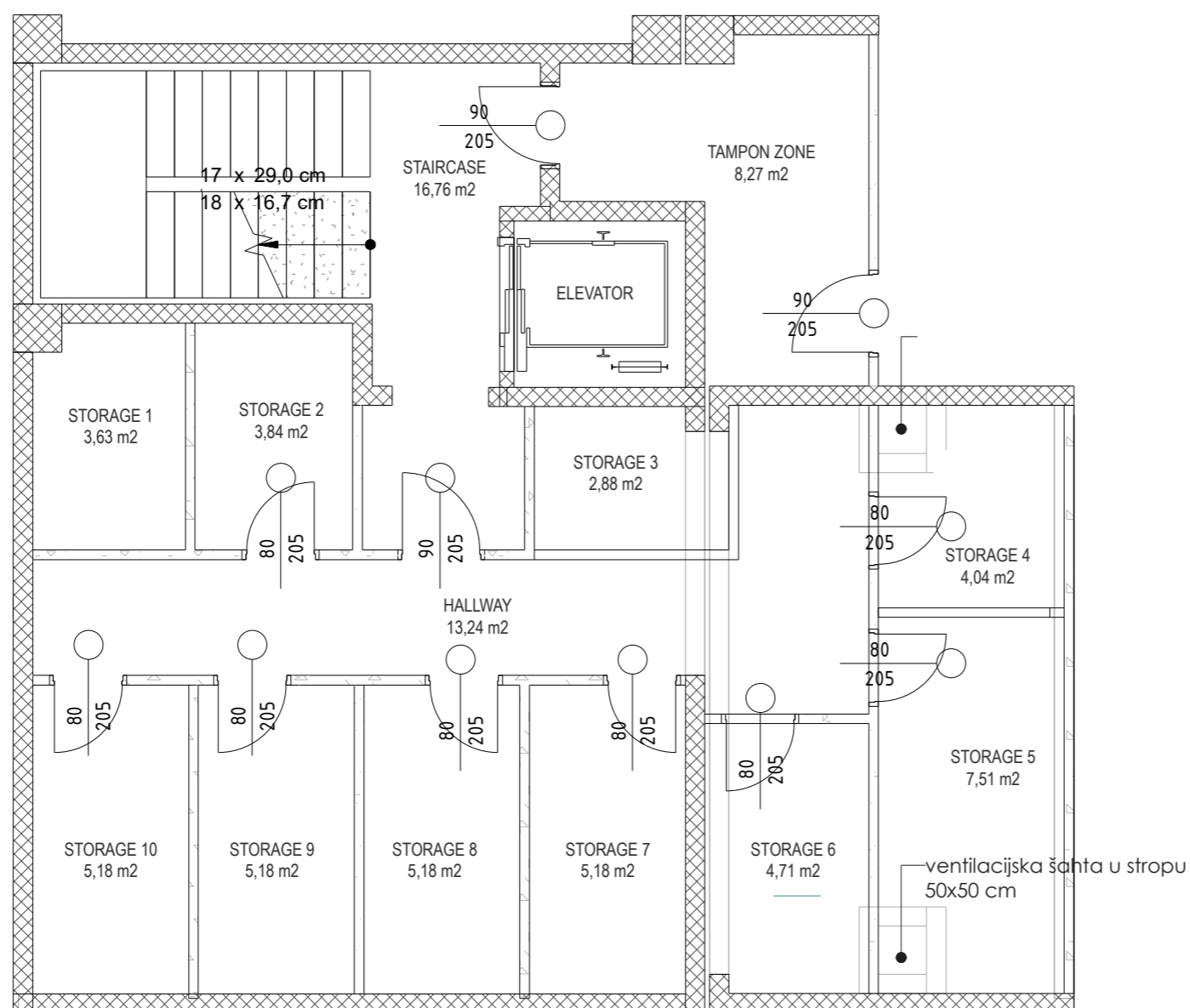
PLAN
