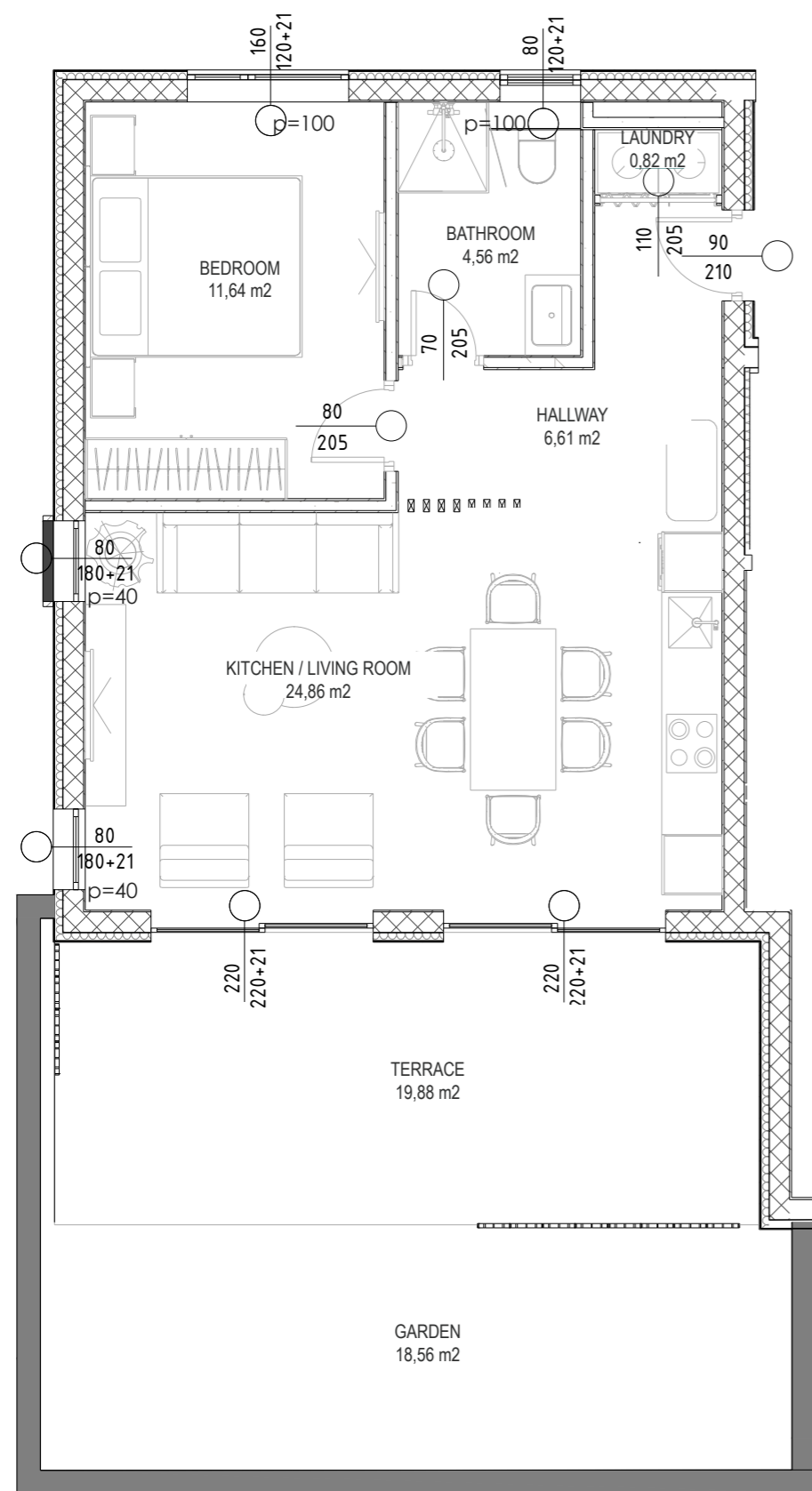
PLAN
