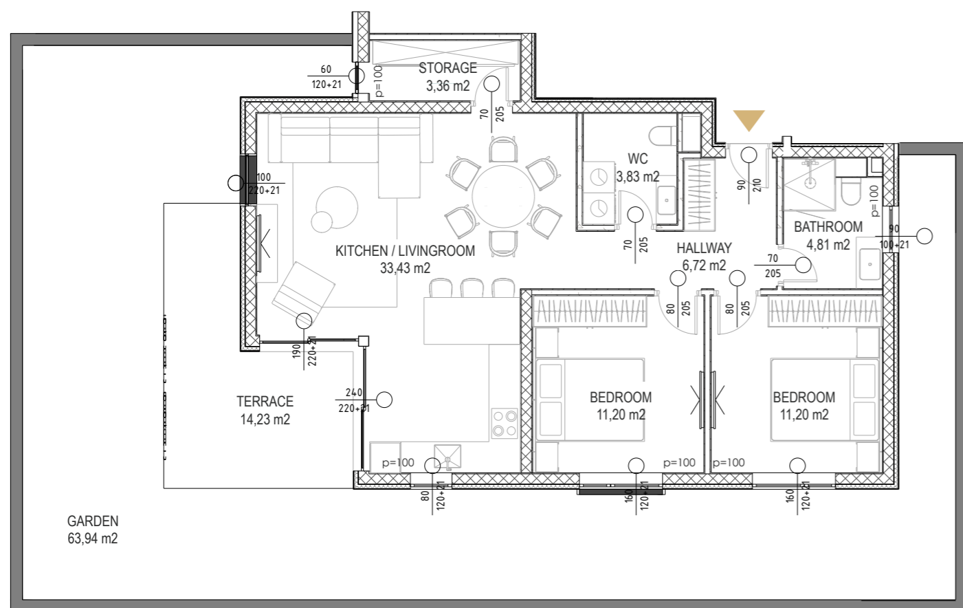
PLAN
