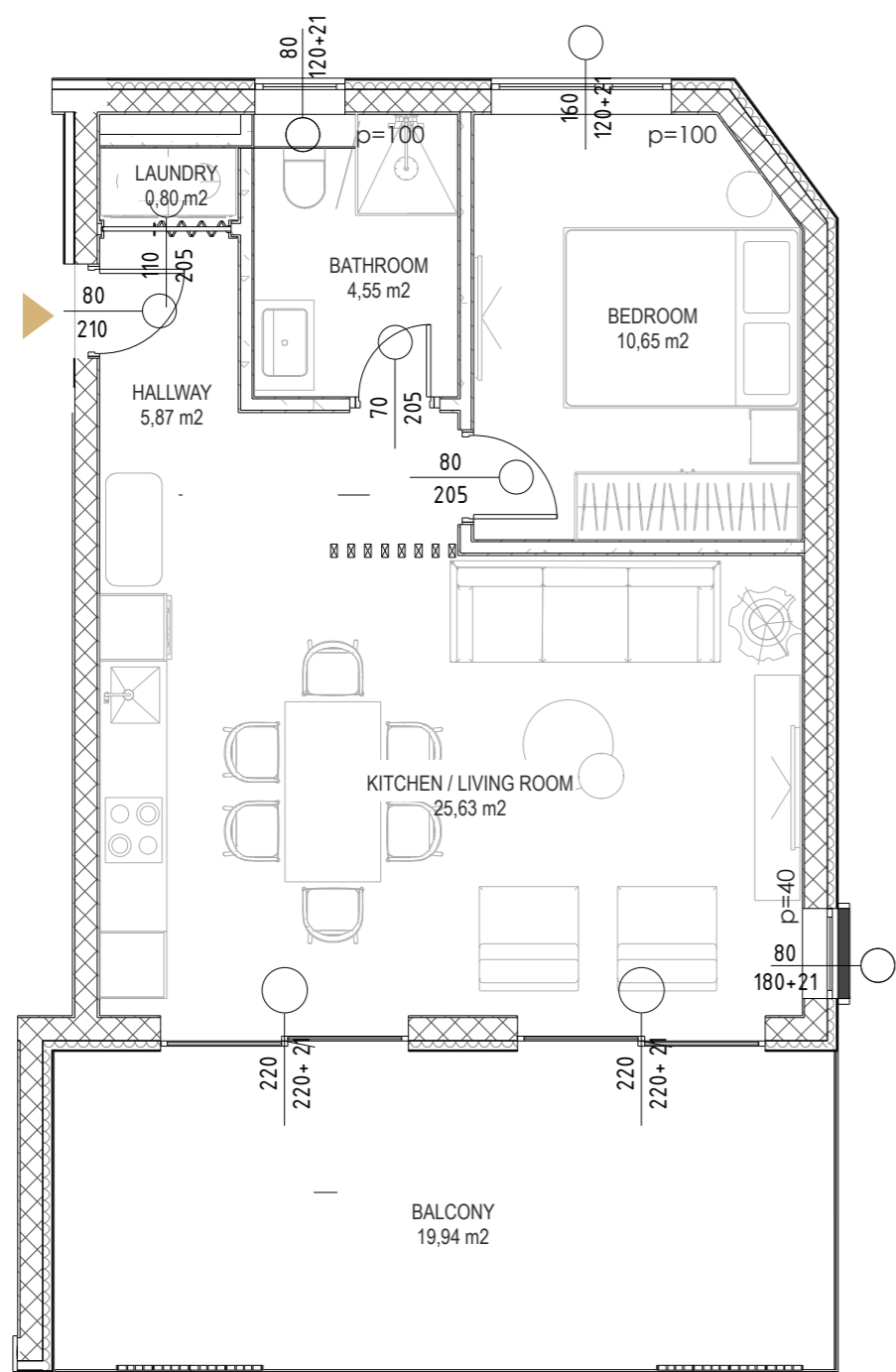
PLAN
