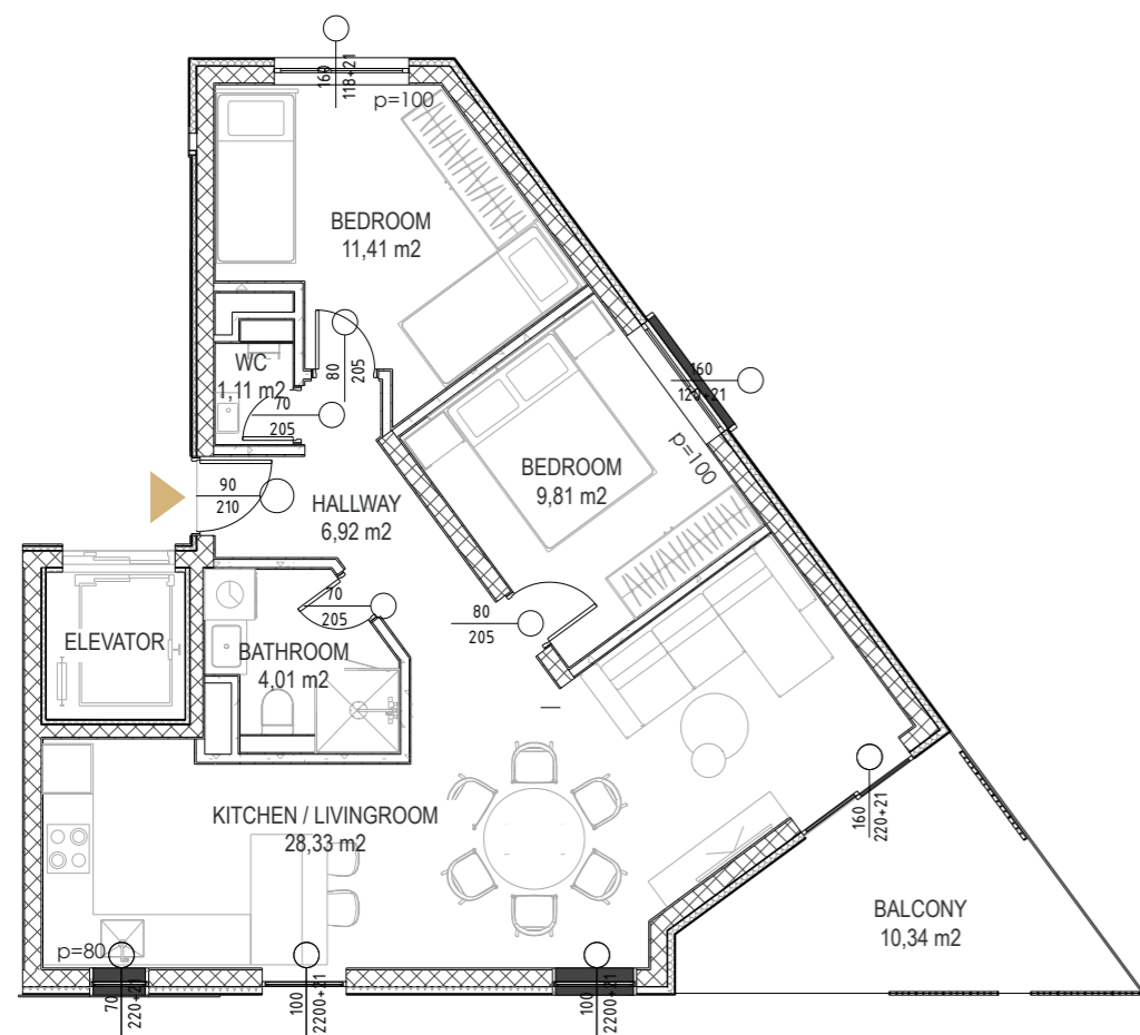
PLAN
